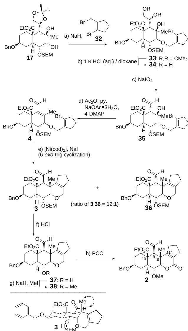
Scheme 5. Synthesis of tetracycles 3 and 36 by Ni 0 -mediated cyclization and further elaboration of 3 to 2 . a) NaH (3.0 equiv), 32 (1.7 equiv), THF, 25 °C, 24 h, 63%; b) dioxane:1 N HCl (aq.) (5:1, 0.01 M), 40 °C, 1 h, 74%; c) NaIO 4 (1.5 equiv), THF/H 2 O (2:1), 25 °C, 24 h, 100%; d) NaOAc·3H 2 O (15.0 equiv), 4-DMAP (3.0 equiv), Ac 2 O/py (1:1), 50 °C, 24 h, 67%; e) [Ni(cod) 2 ] (6.0 equiv), NaI (10.0 equiv), DMF, 80 °C, 2 h, 55%; f) 1 N HCl (aq.) in dioxane (3:1), 50 °C, 6 h, 85%; g) NaH (10.0 equiv), MeI (10.0 equiv), THF, 50 °C, 2 h, 89%; h) PCC (5.0 equiv), CH 2 Cl 2 , 50 °C, 24 h, 79% at 56% conversion. PCC = pyridinium chlorochromate.
