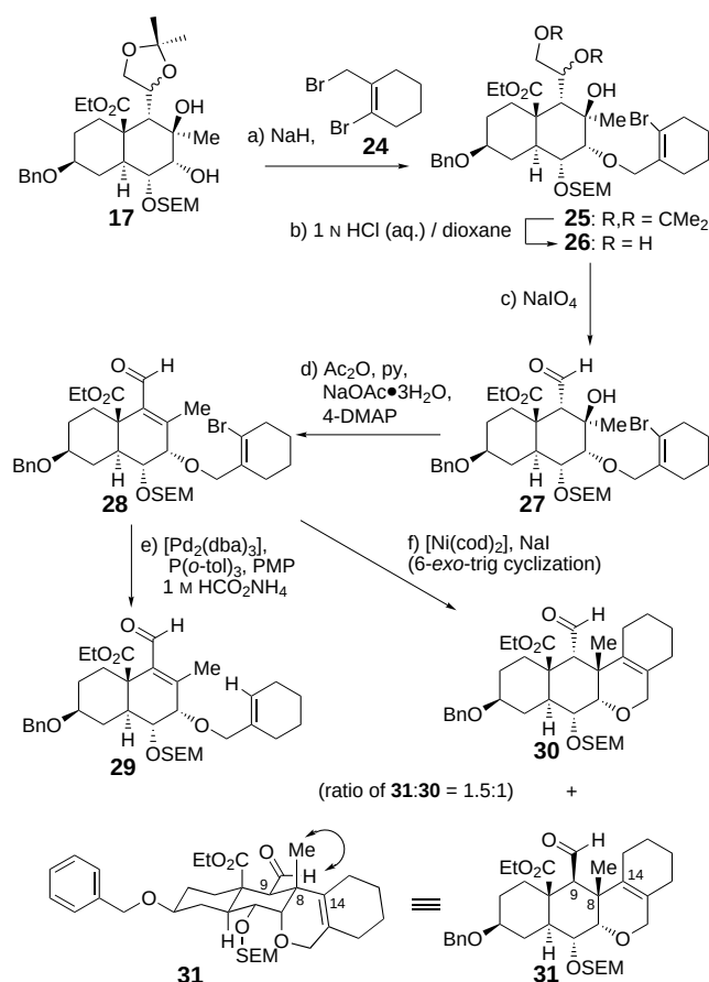
Scheme 4. Synthesis of tetracycles 30 and 31 by Ni 0 -mediated cyclization. a) NaH (3.0 equiv), 24 (1.7 equiv), THF, 25 °C, 24 h, 60%; b) dioxane:1 N HCl (aq.) (5:1, 0.01 M), 40 °C, 1 h, 74%; c) NaIO 4 (1.5 equiv), THF/H 2 O (2:1), 25 °C, 24 h, 100%; d) NaOAc·3H 2 O (15.0 equiv), 4-DMAP (3.0 equiv), Ac 2 O/py (1:1), 50 °C, 24 h, 70%; e) [Pd 2 (dba) 3 ] (0.5 equiv), P(o-tol) 3 (1.0 equiv), PMP (10.0 equiv), toluene/THF/1 M HCO 2 NH 4 (aq.) (6:2:1), 60 °C, 11 h, 100%; f) [Ni(cod) 2 ] (6.0 equiv), NaI (10.0 equiv), DMF, 80 °C, 2 h, 60%. cod = 1,5-cyclooctadiene.
