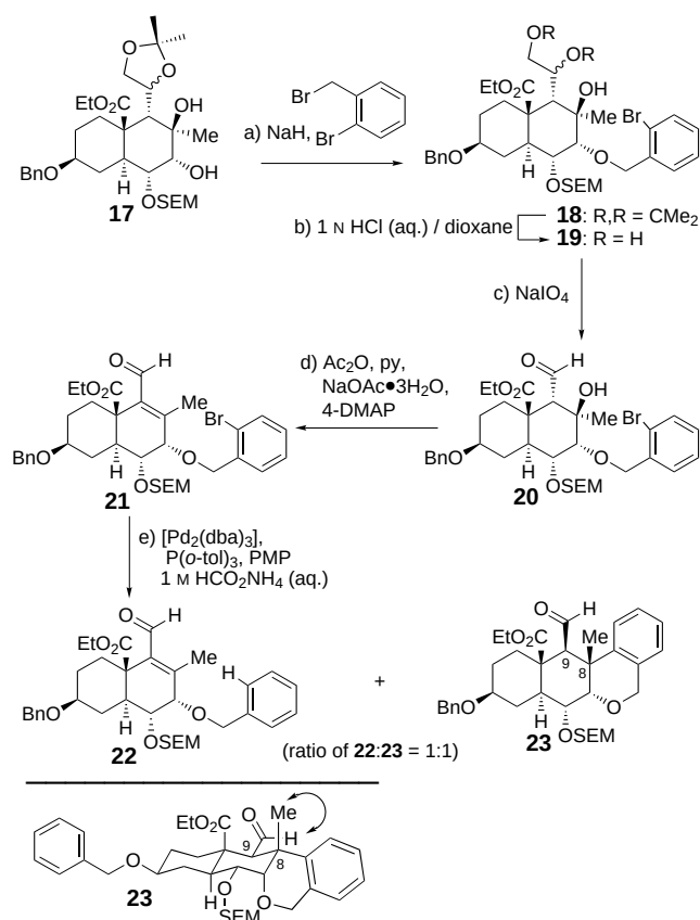
Scheme 3. Synthesis of tetracycle 23 via Pd 0 -catalyzed cyclization. a) NaH (3.0 equiv), 2-bromobenzyl bromide (1.7 equiv), THF, 25 °C, 24 h, 75 %; b) dioxane:1N HCl (aq.) (5:1, 0.01M), 40 °C, 1 h, 80 %; c) NaIO 4 (1.5 equiv), THF/H 2 O (2:1), 25 °C, 24 h, 100 %; d) NaOAc·3H 2 O (15.0 equiv), 4-DMAP (3.0 equiv), Ac 2 O/py (1:1), 50 °C, 24 h, 73 %; e) [Pd 2 (dba) 3 ] (0.5 equiv), P( o -tol) 3 (1.0 equiv), PMP (10.0 equiv), toluene/THF/1M HCO 2 NH 4 (aq.) (6:2:1), 60 °C, 11 h, 100 %. dba = dibenzylideneacetone, 4-DMAP = 4-dimethylaminopyridine, PMP = 1,2,2,6,6-pentamethylpiperidine, py = pyridine.
